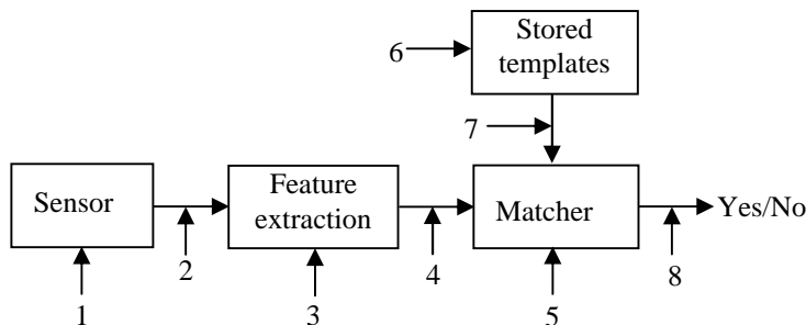
Figure 1: Attack points of a biometric system
